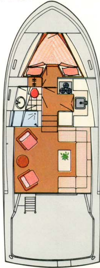
STANDARD LOWER GALLEY ARRANGEMENT features full-sized salon, lower level galley, bow stateroom.
