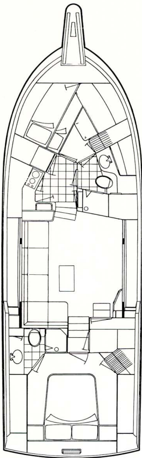
STANDARD ARRANGEMENT 40 MY
