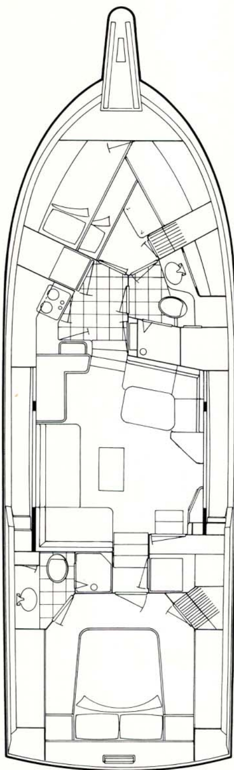
OPTIONAL ARRANGEMENT 40MY
