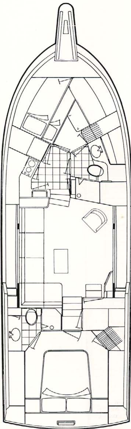
STANDARD ARRANGEMENT
