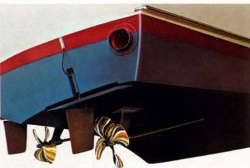
Special feature of this 38 is the deep keel for better protection of running gear. It is an aid to a more stabilized ride, as are the standard adjustable tabs as shown.
