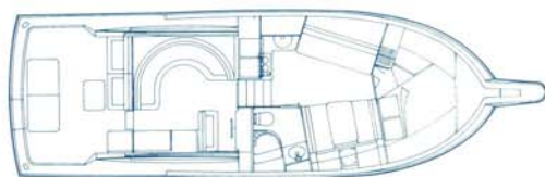
CURVED BRIDGE SEATING WITH AFT FACING LOUNGE IN THE COCKPIT.
