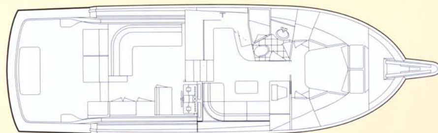
STANDARD ARRANGEMENT*
