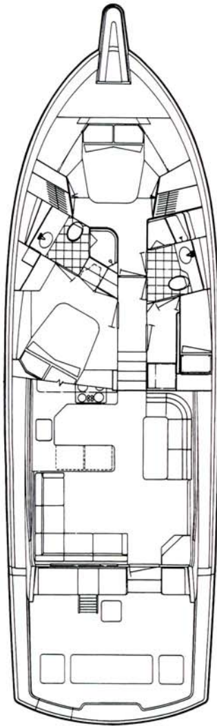
STANDARD ARRANGEMENT
