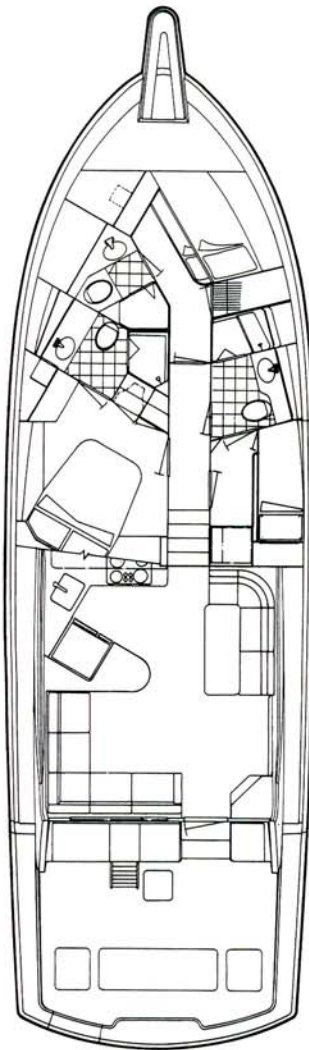
OPTIONAL BOW STATEROOM AND GALLEY
