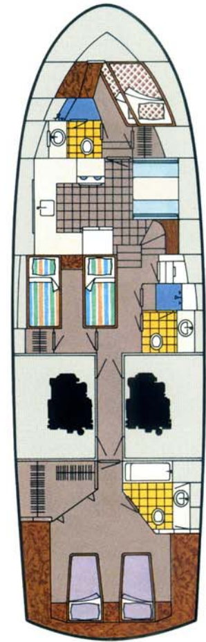
Floor plan with optional twin berth/master stateroom arrangement.
