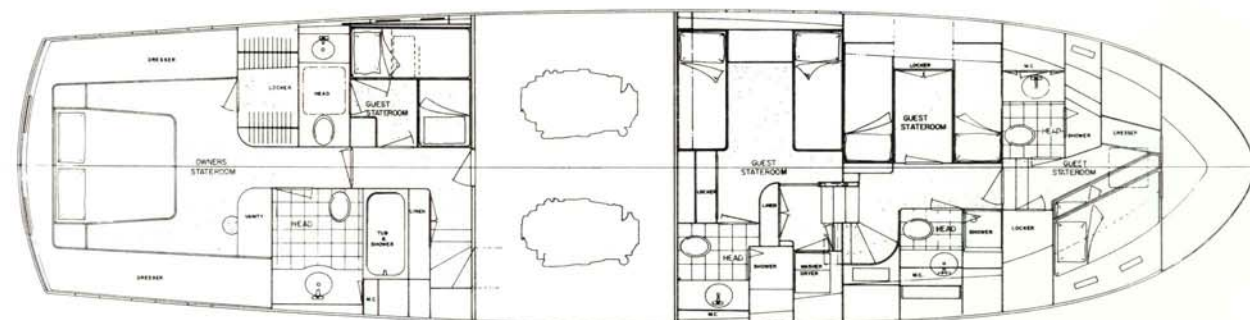
OPTIONAL ARRANGEMENT
