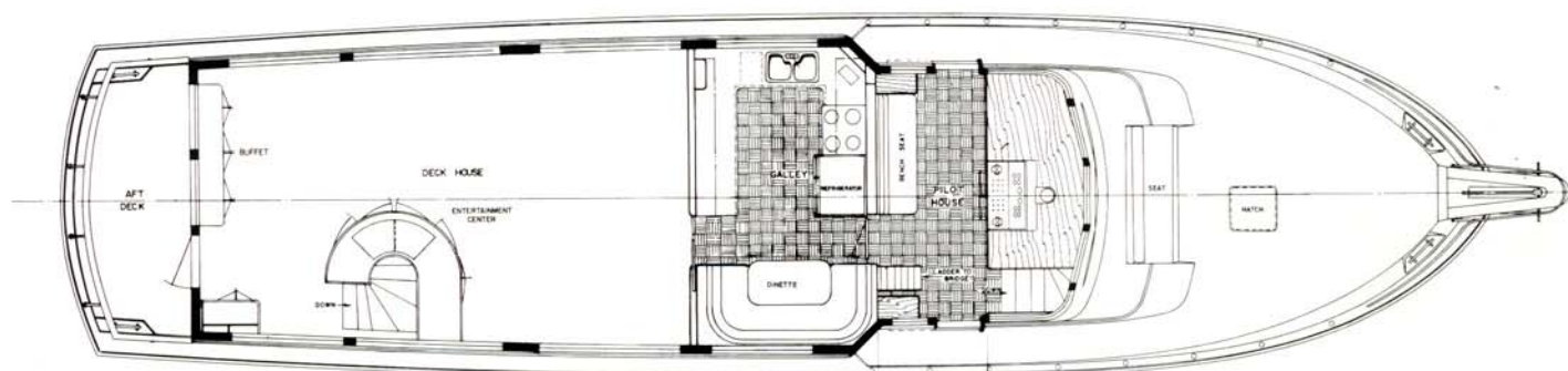
DECKHOUSE ARRANGEMENT
