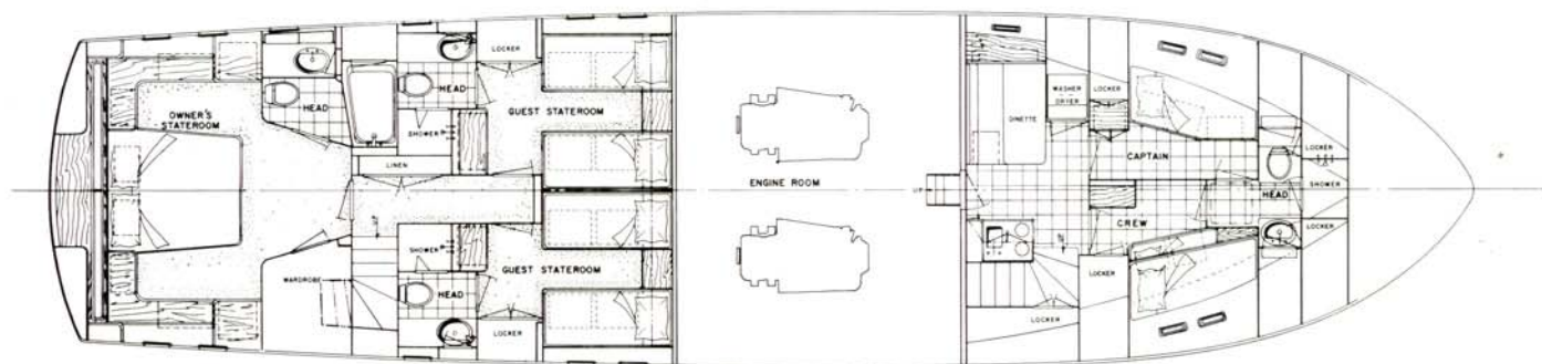
LOWER DECK ARRANGEMENT
